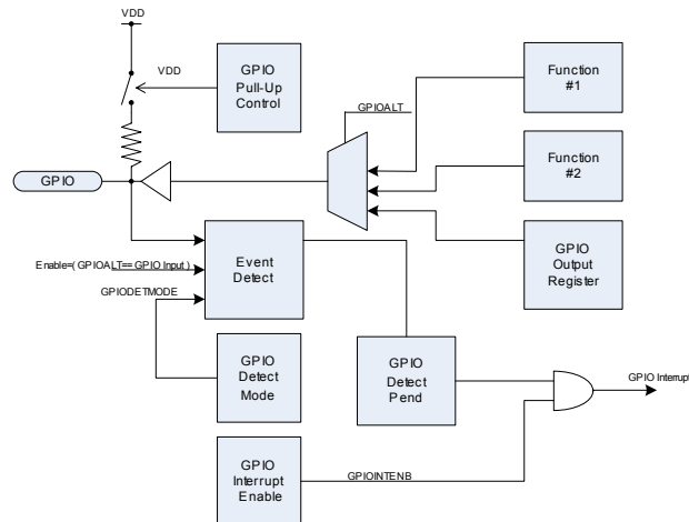
Figure 7-1 GPIO Data path block diagram
