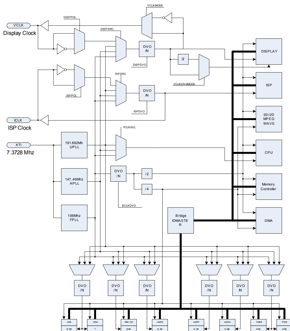
Figure 5.1 Clock Path diagram
